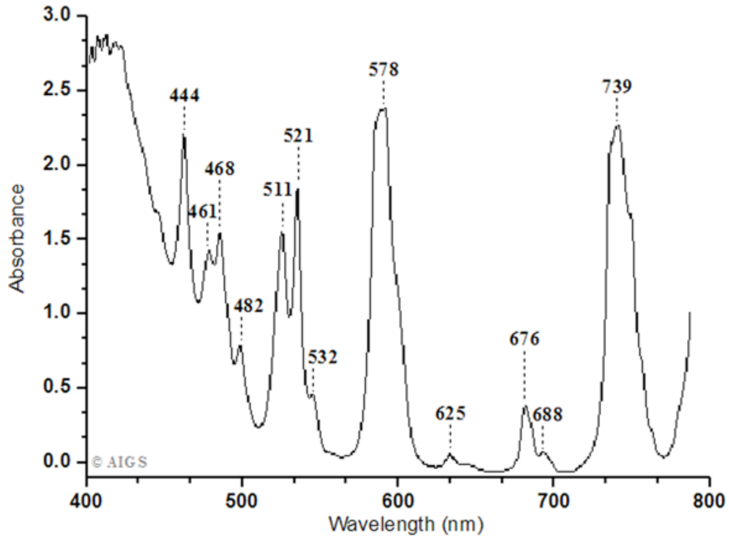
Visible spectrum of the 2.09 ct color-change Bastnäs site - Pakistan
