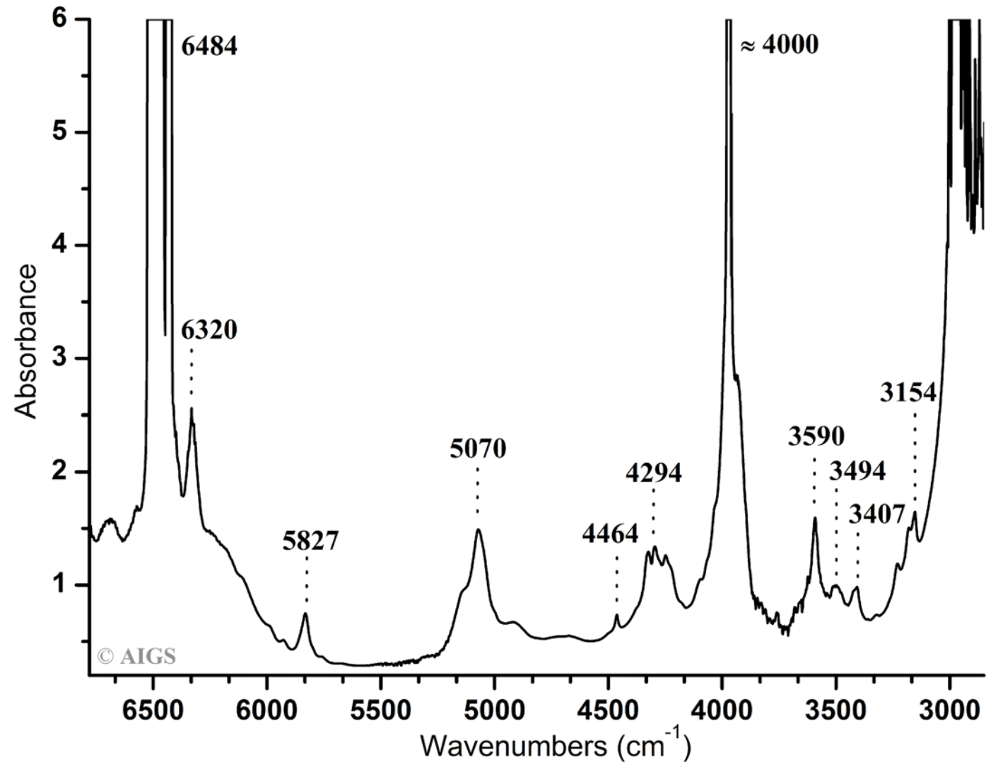
Infrared spectrum of the 2.09 ct color-change Bastnäs site - Pakistan
