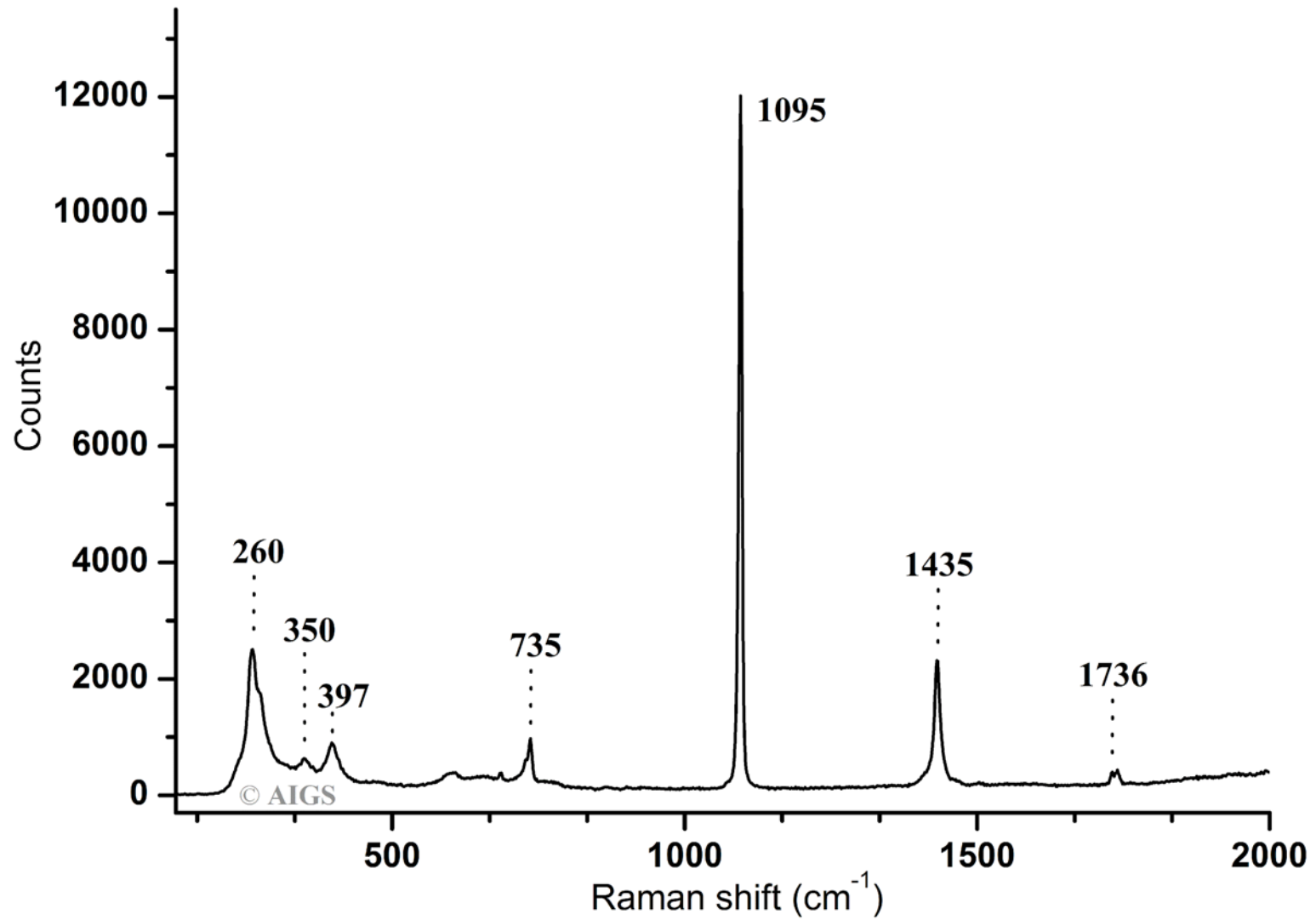
Raman spectrum of the 2.09 ct color-change Bastnäs site - Pakistan
